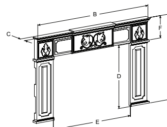
SC(25/33)6BL 6 x 6-inch Cast Iron Surround
