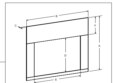
SH1BL Universal Shroud (for insert installations only, drawing not to scale)
